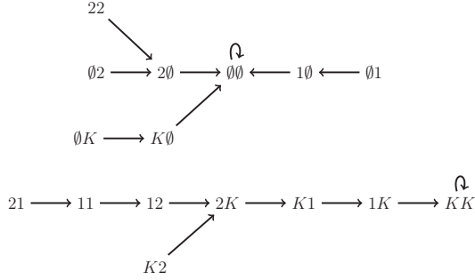
FIG. 3.3. The phase space \mathcal{PS}_f for the Boolean 2-linear map f on K = [2] indicated in Fig. 3.2.
