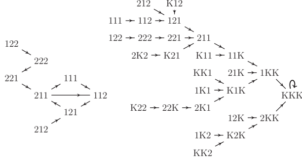
FIG. 3.5. The digraph and part of the phase space of the 3-linear map in Example 3.5.
