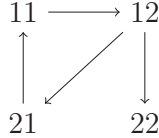
FIG. 3.2. The digraph \Gamma_f of a Boolean 2-linear map f on K = [2] .
