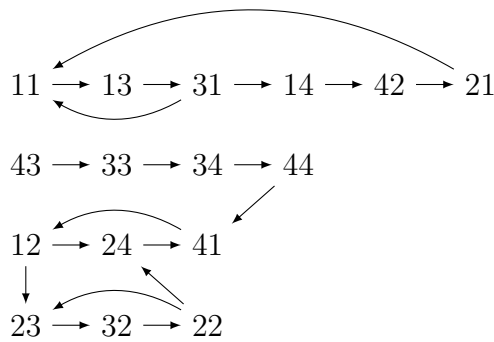
Figure 5: The De Bruijn form \Gamma_f of a 2-hydra f on [4] .
